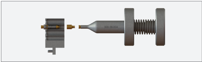
Figure 11.1 Bullet Installation to Contact. Uses Tool PN 500-38-004.
