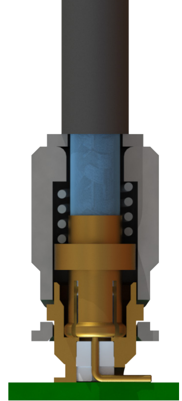
Figure 3: Cut-away view of a mated Female QB Cable Assembly to Male QB PCB Connector
